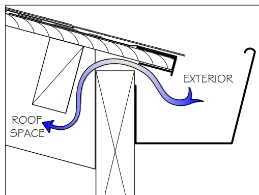
AIR-FLOW DIAGRAM @ 1:5
