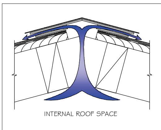
AIR-FLOW DIAGRAM @ 1:5
