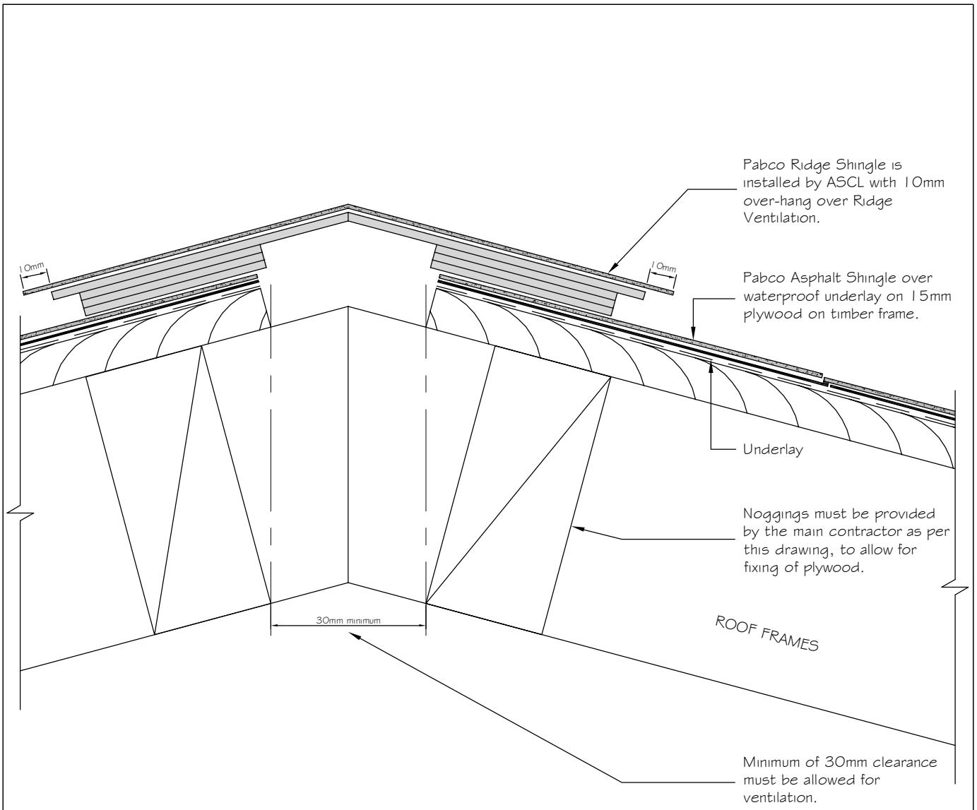
AIR-FLOW DIAGRAM @ 1:5
